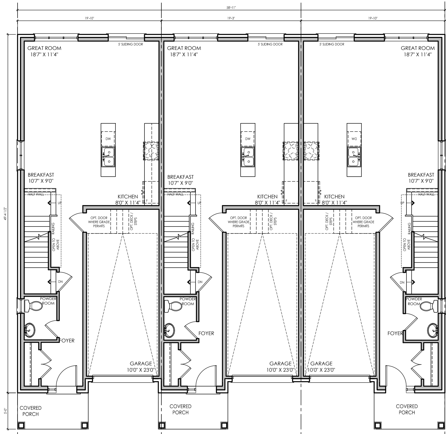
GROUND FLOOR Floor Area: 719 s.f.
